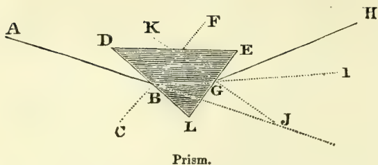
Prism.
